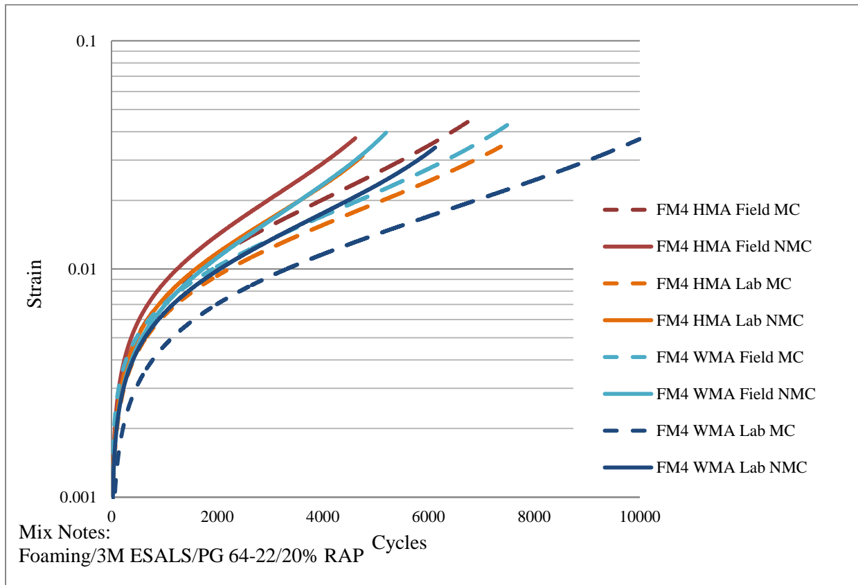
Figure 4.15 Strain versus cycles plot for FM4 (HMA/Foam)
