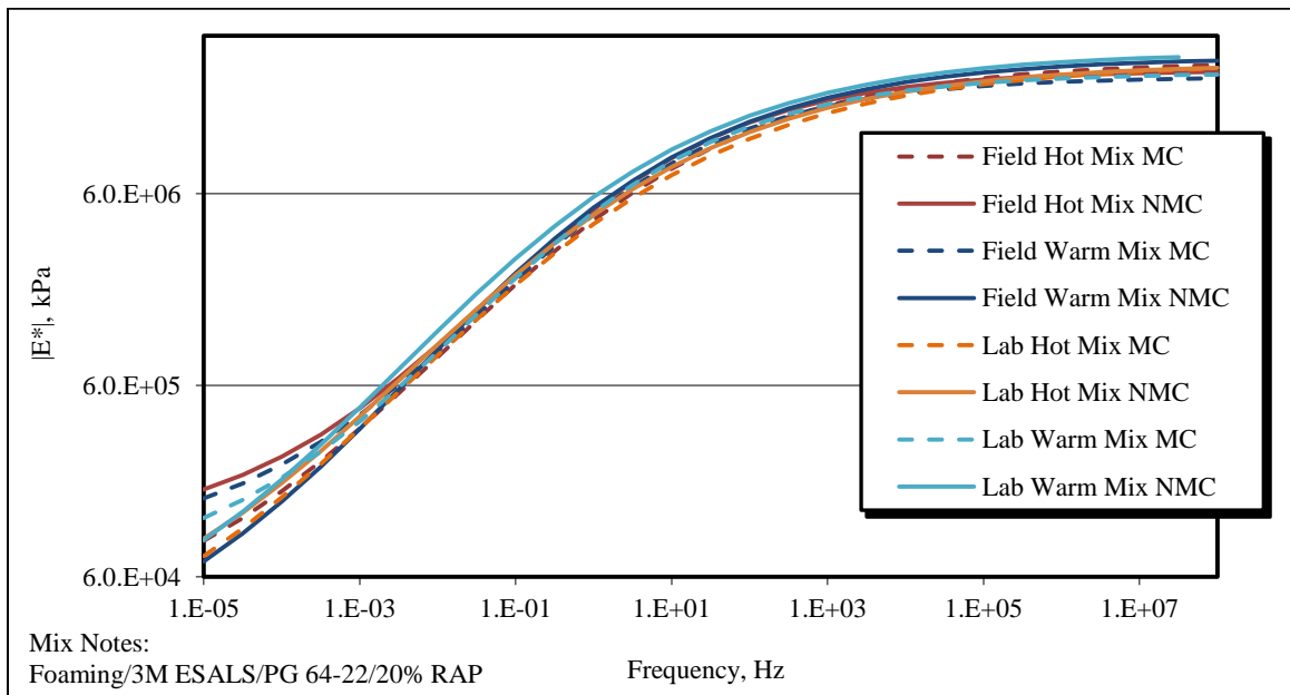
Figure 4.6 FM4 (HMA/Foaming) dynamic modulus master curves
