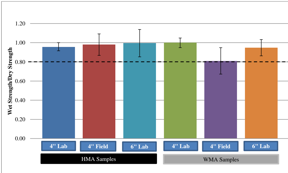
Figure 4.31 FM3 TSR results (HMA/Sasobit)
