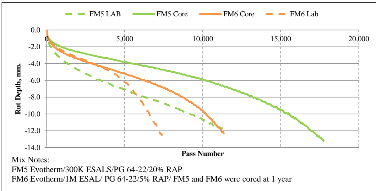
Figure 4.43 FM5 and FM6 Hamburg rutting depth versus passes (Evotherm) (Average core air voids are FM5=11.3% and FM6=7.1%)
