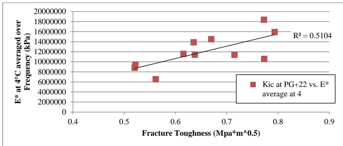
Figure 7.7 Dynamic modulus at 4^\circ\text{C} compared with fracture toughness at PG+22
