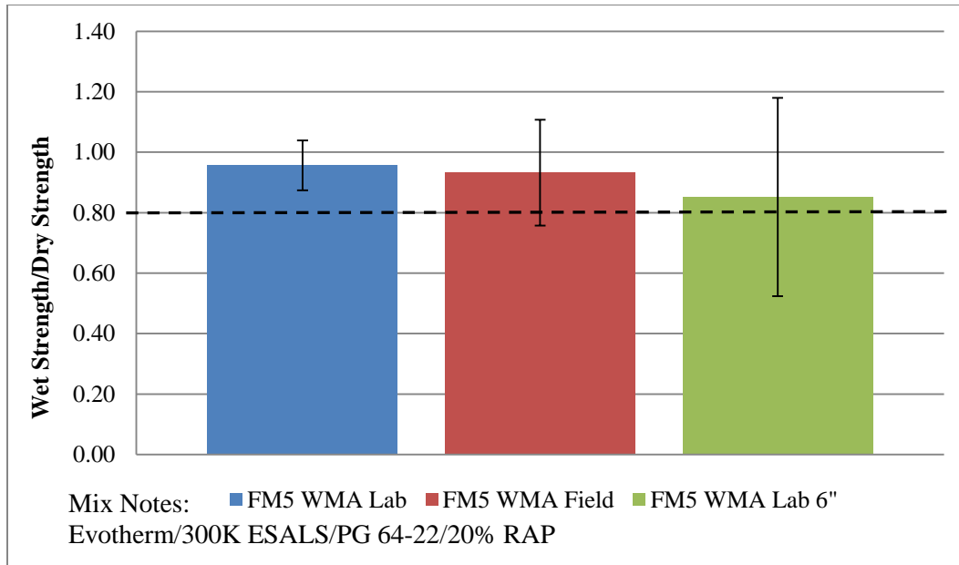
Figure 4.35 Tensile Strength Ratio for FM5
