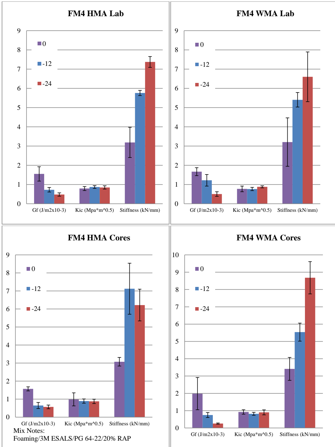
Figure 4.24 SCB results for FM4 (HMA/Foam) (Average core air voids are HMA=4.3% and WMA=3.45%; pavement cored after 2 years of service life)
