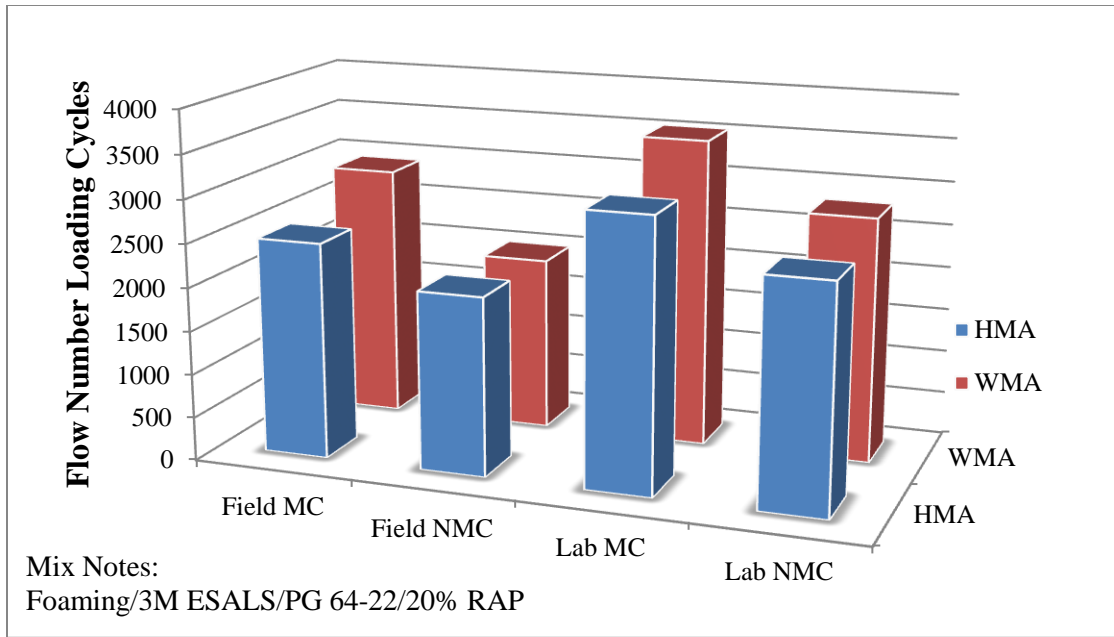
Figure 4.14 Flow number comparisons for FM4
