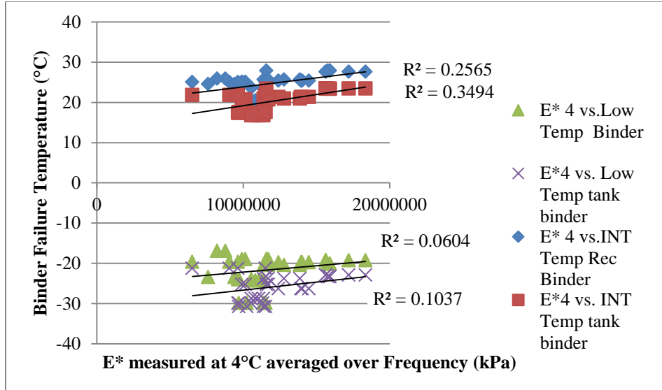
Figure 7.1 Binder properties compared with dynamic modulus at 4°C
