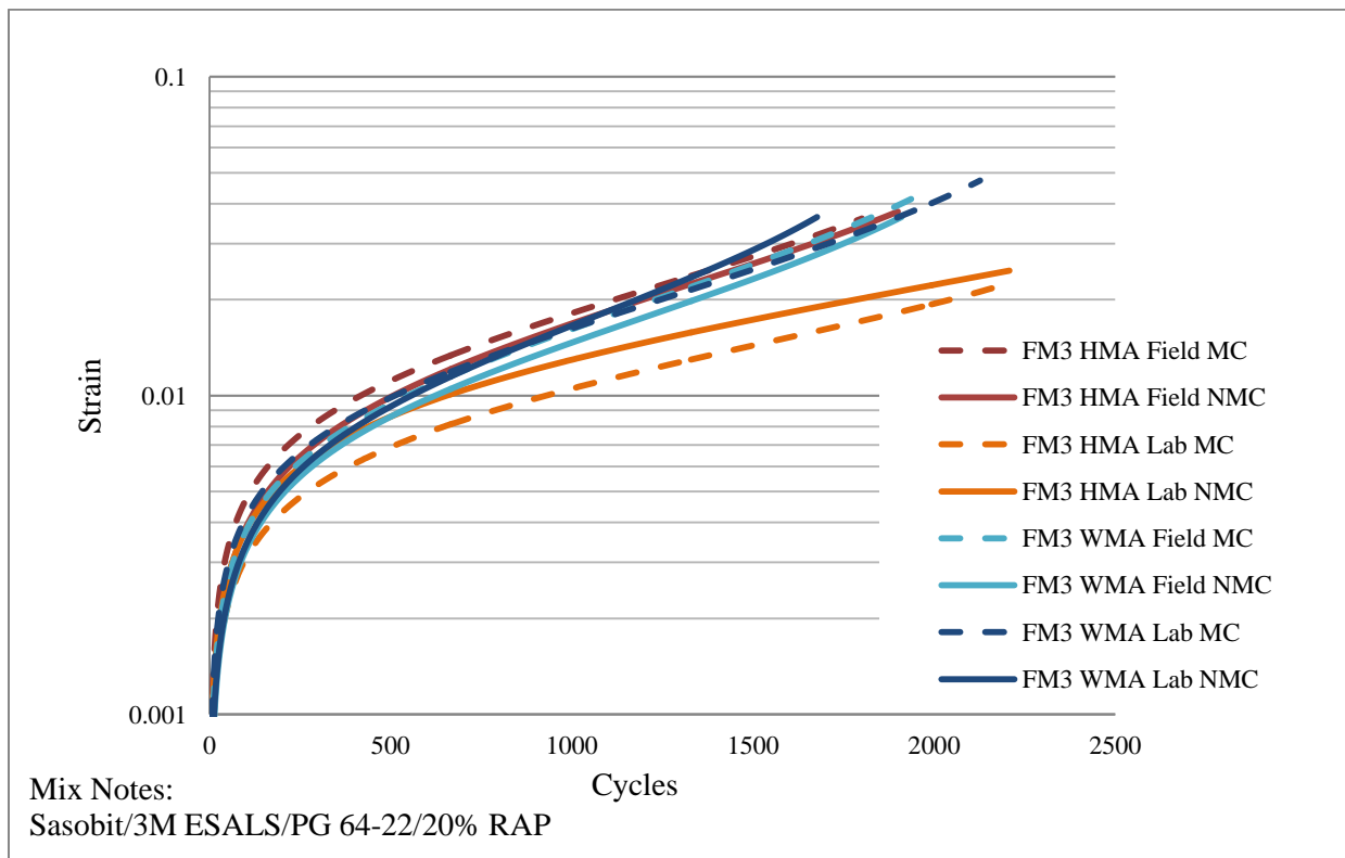
Figure 4.13 Strain versus cycles plot for FM3 (HMA/Sasobit)
