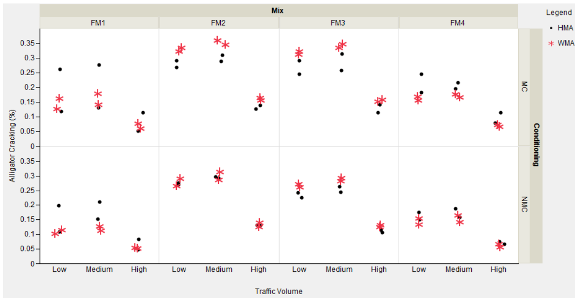
Figure 6.5 MEPDG predicted alligator cracking
