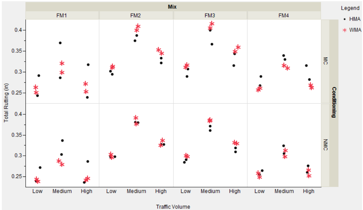
Figure 6.6 MEPSDG predicted total rutting
