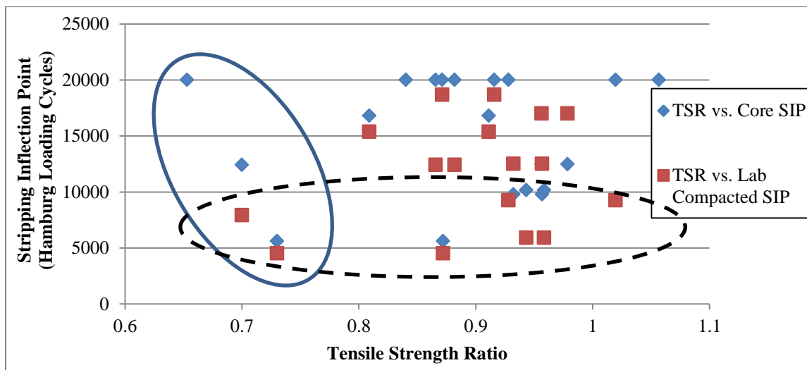
Figure 7.11 Relationship of tensile strength ratio and stripping inflection point
