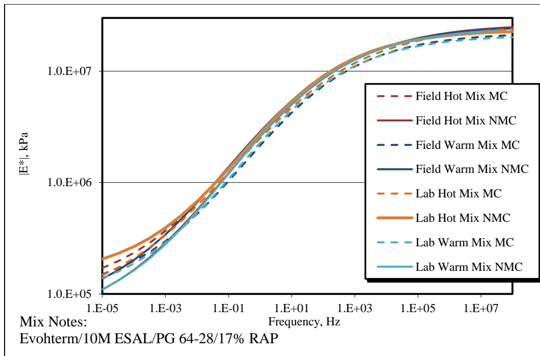
Figure 4.4 FM2 (HMA/Evotherm) dynamic modulus master curves
