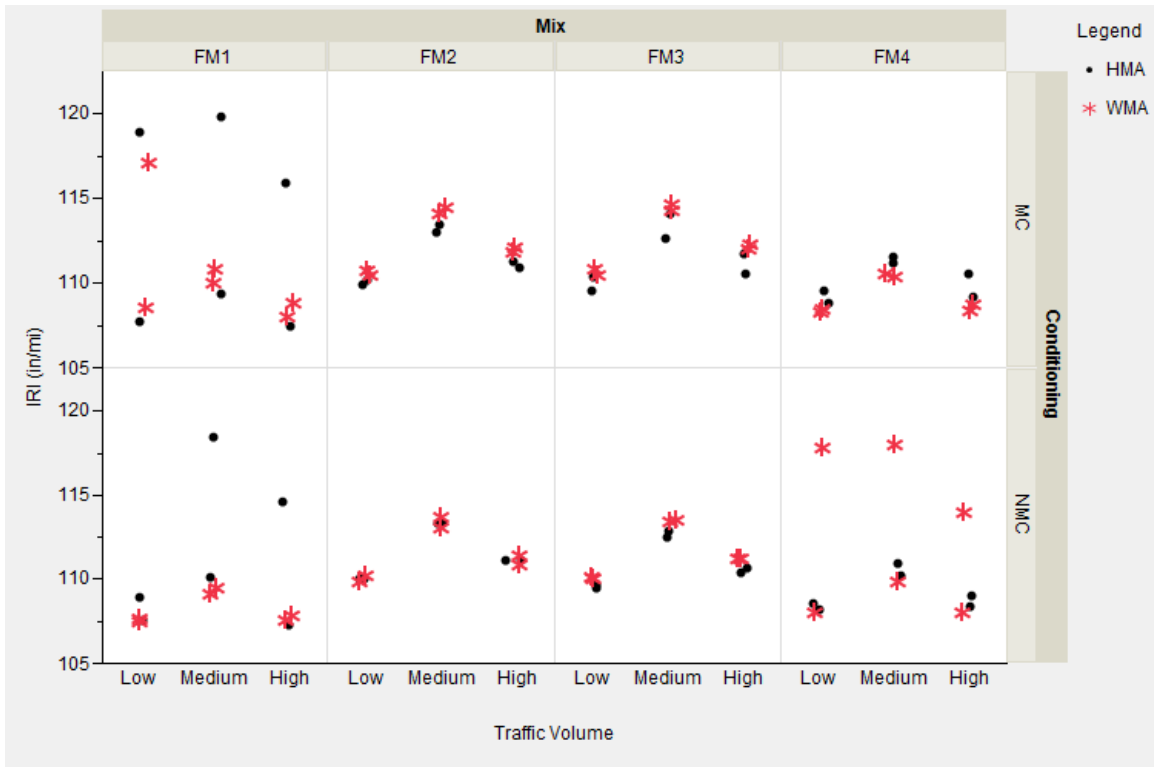
Figure 6.7 MEPSDG predicted IRI
