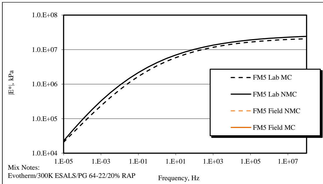
Figure 4.7 FM5 (Evotherm only) dynamic modulus master curves
