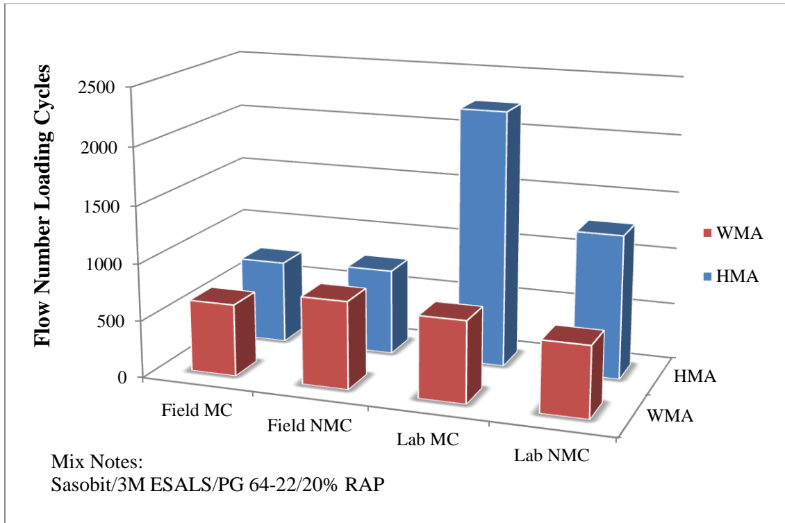
Figure 4.12 FM3 flow number comparison
