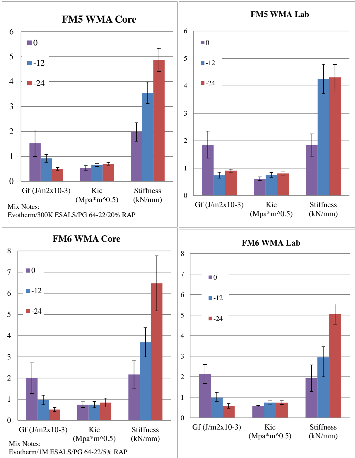
Figure 4.25 SCB results for FM5 and FM6 (Evotherm)
