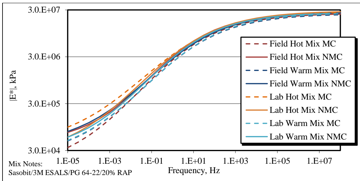
Figure 4.5 FM3 (HMA/Sasobit) dynamic modulus master curves
