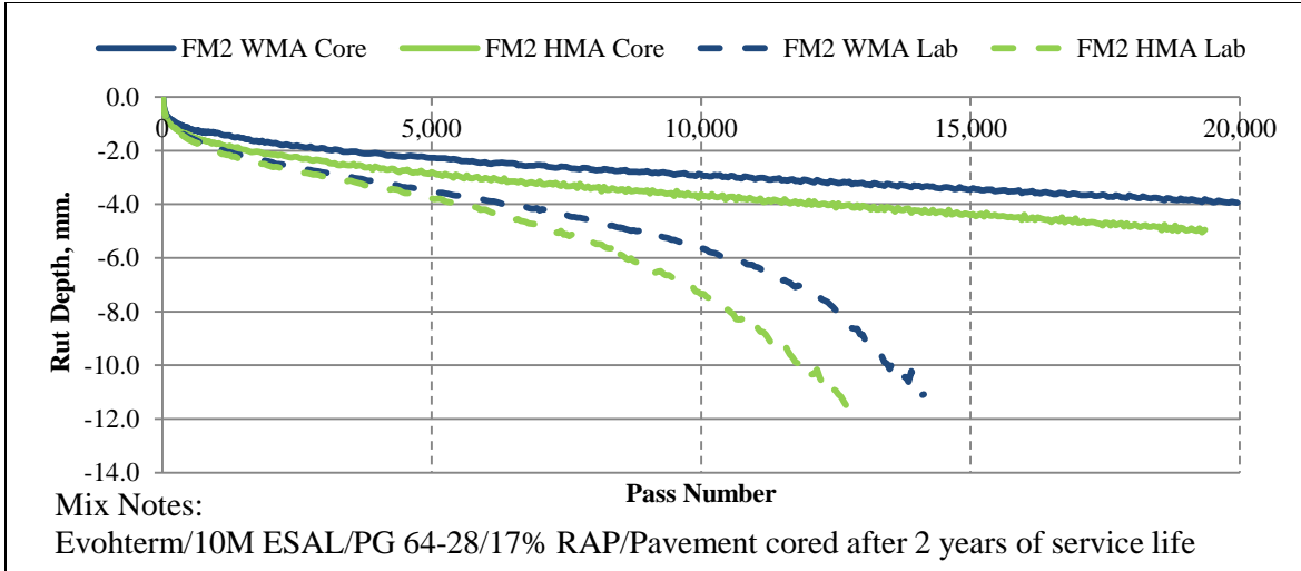
Figure 4.40 FM2 Hamburg rutting depth versus passes (HMA/Evothertm) (Average core air voids are HMA=7.3% WMA=7.1%)
