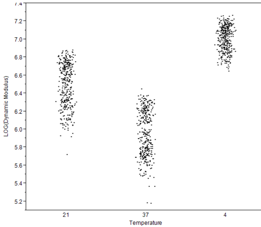
Figure 4.3 Dynamic modulus data with a log transformation
