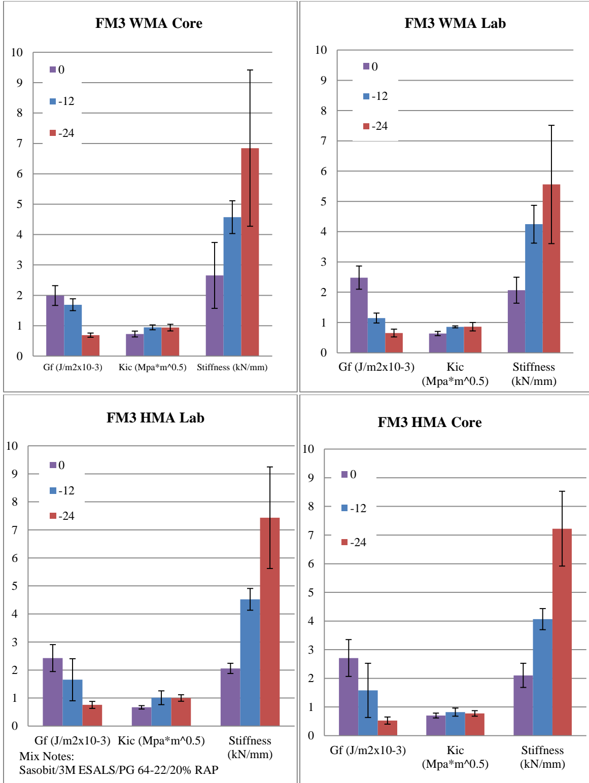
Figure 4.23 SCB results for FM3 (HMA/Sasobit)
