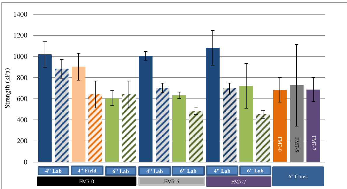
Figure 4.38 FM7 IDT peak strength (Evotherm with 0%, 5%, and 7% Shingles) (Age of cores is 1 year. Average core air voids are FM7-0=8.0%, FM7-5=8.6% and FM7-7=10.6%)
