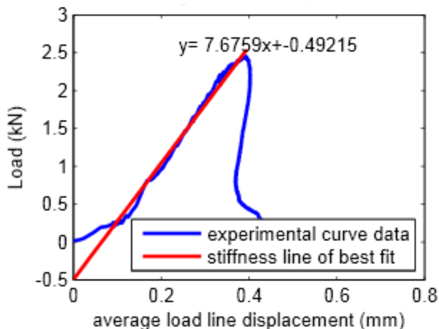
Figure 3.8 Example graph showing how stiffness is calculated
