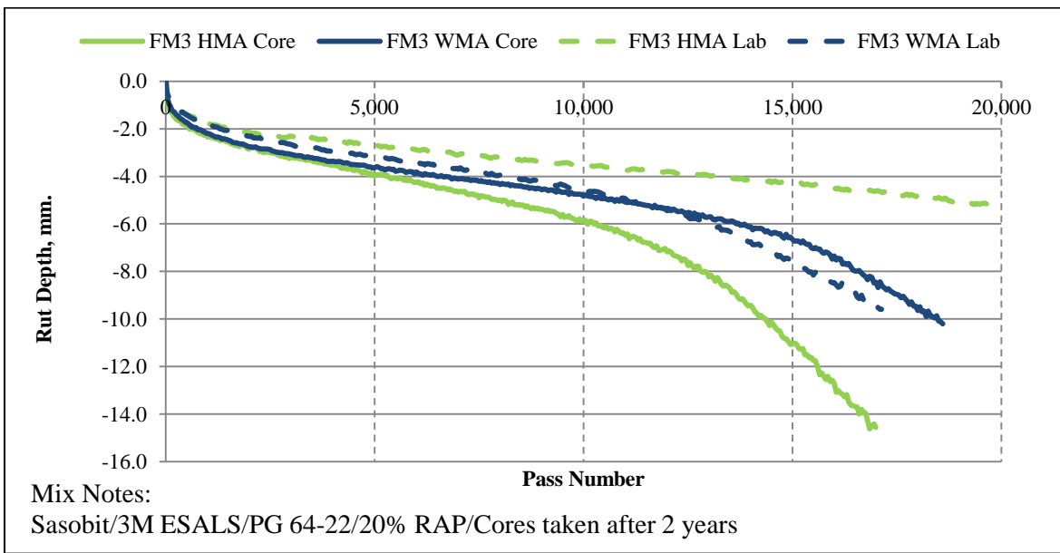
Figure 4.41 FM3 Hamburg rutting depth versus passes (HMA/Sasobit) (Average core air voids are HMA=8.2% and WMA=7.8%)
