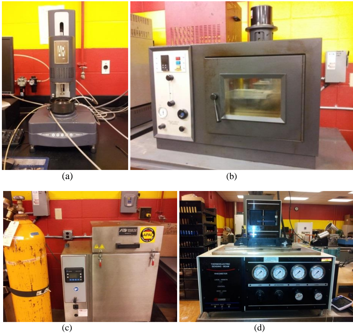
Figure 3.11 Binder testing equipment (a) Dynamic shear rheometer (b) Rolling thin film oven (c) Pressure aging vessel (d) Bending beam rheometer
