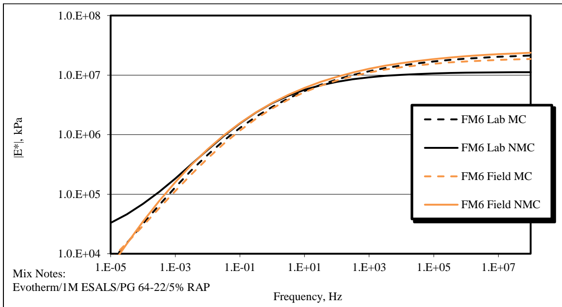
Figure 4.8 FM6 (Evotherm) dynamic modulus master curves
