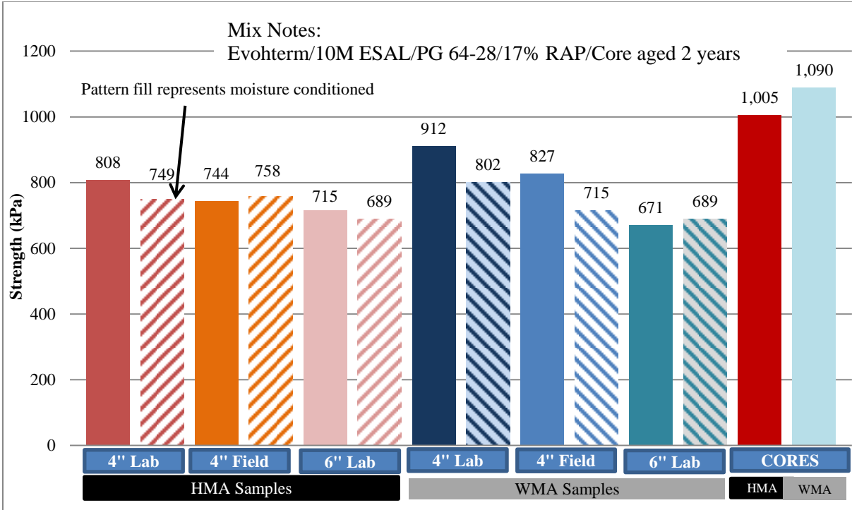
Figure 4.28 FM2 IDT peak strength (HMA/Evotherm) (Average core air voids are HMA=3.4% and WMA=7.6%)
