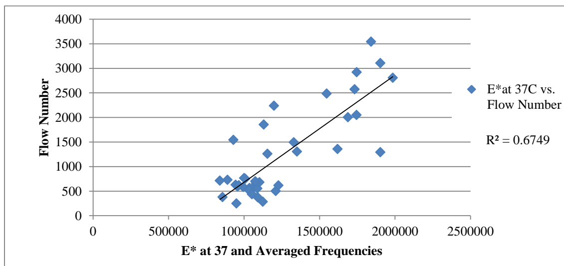
Figure 7.14 Relationship of flow number and high temperature dynamic modulus
