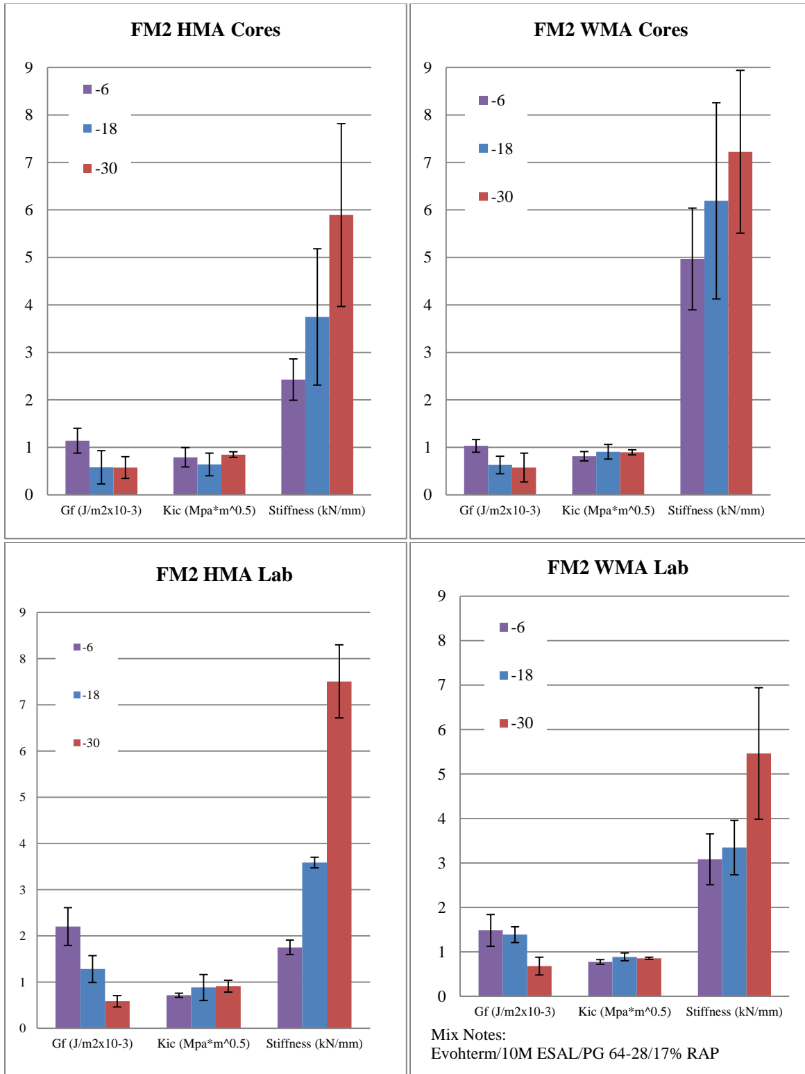
Figure 4.22 SCB results for FM2 (HMA/Evotherm) (Average core air voids are HMA=7.6% and WMA=8.6%; pavement cored after 2 years of service life)
