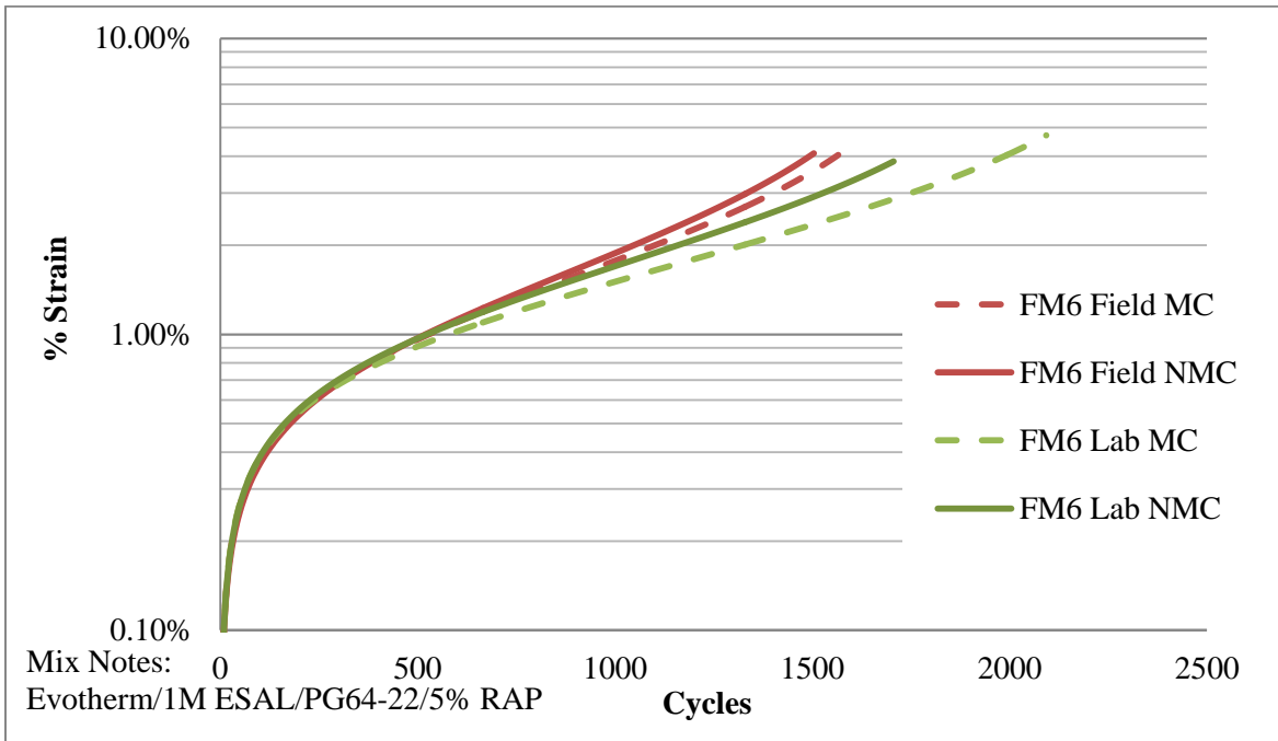
Figure 4.19 Strain versus cycles plot for FM6 (Evotherm)
