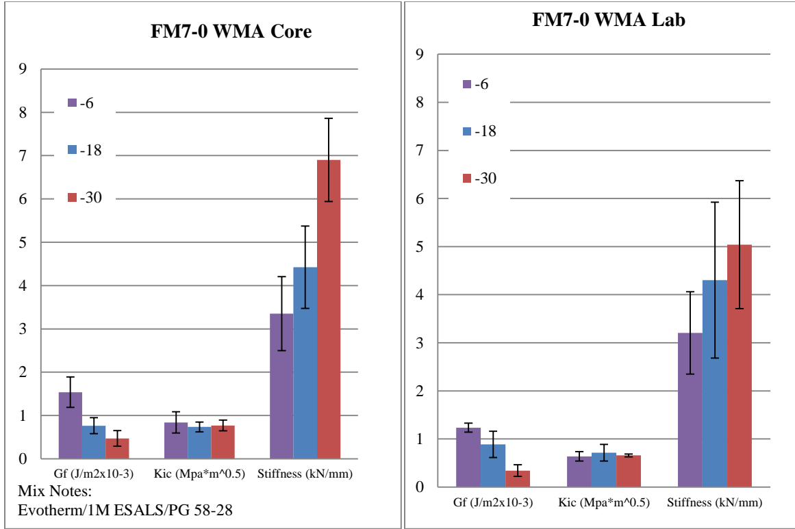
Figure 4.26 SCB results for FM7-0 (Evotherm with 0% Shingles)
