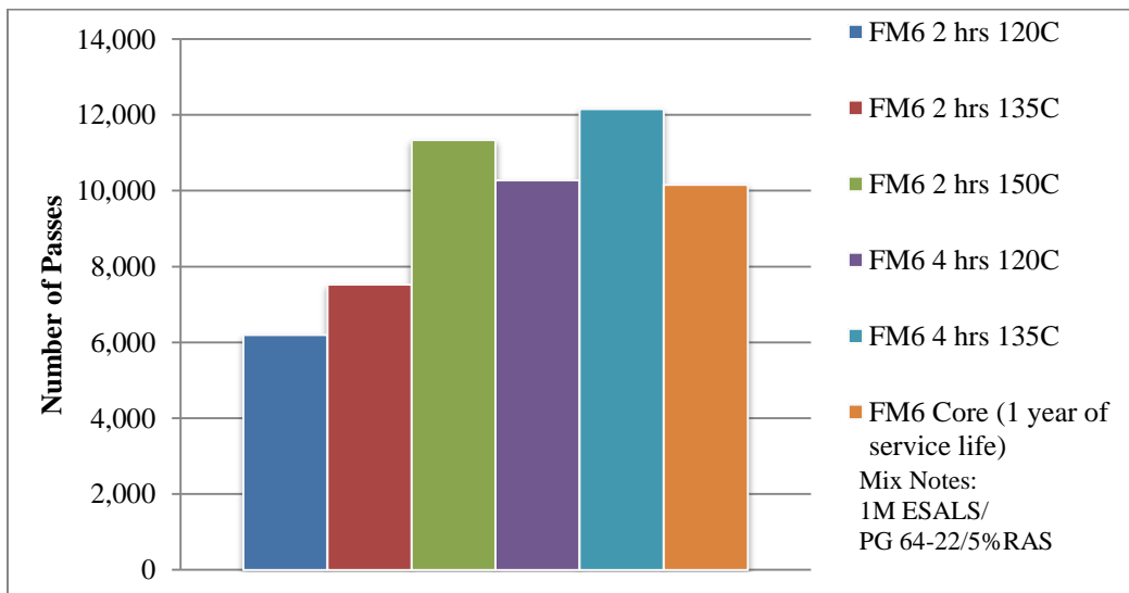
Figure 4.50 Stripping inflection point for FM6 comparing curing time and temperature (Average core air voids are 7.1%)
