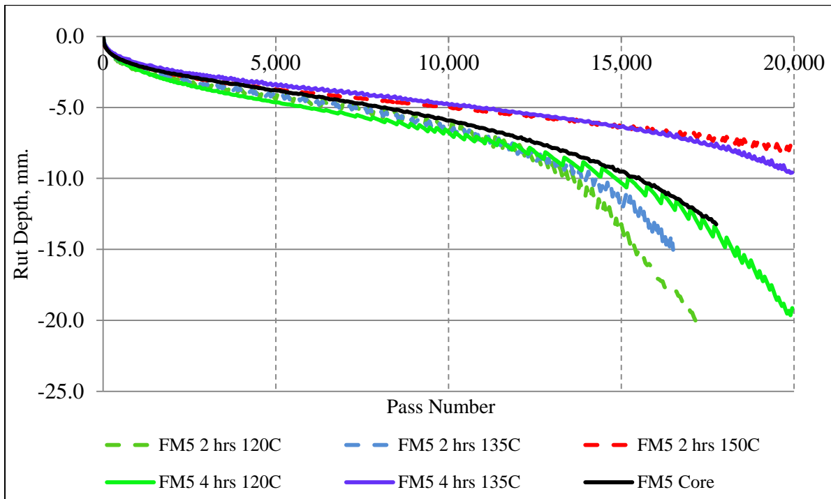
Figure 4.47 FM5 Hamburg wheel tracking test results with variable time and temperatures (Average core air voids are 11.3%)
