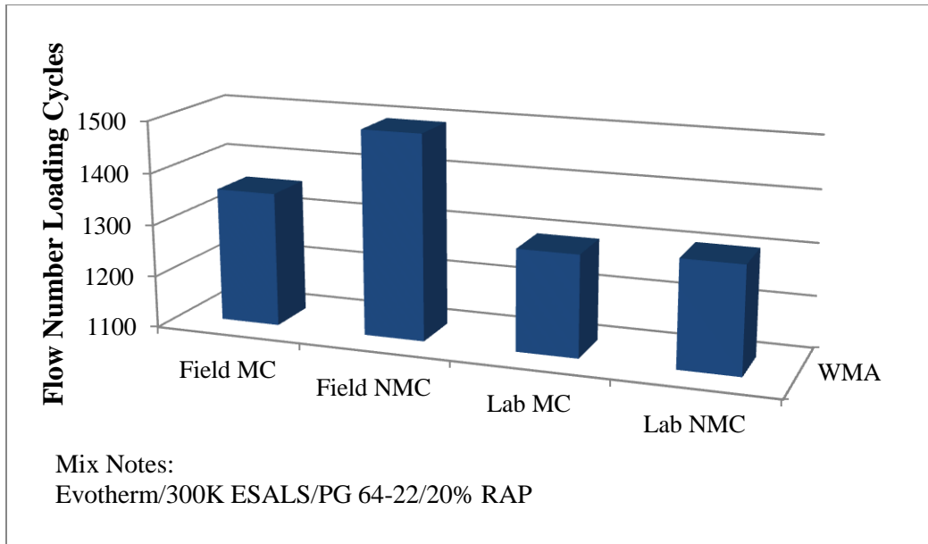
Figure 4.16 Flow number comparison for FM5
