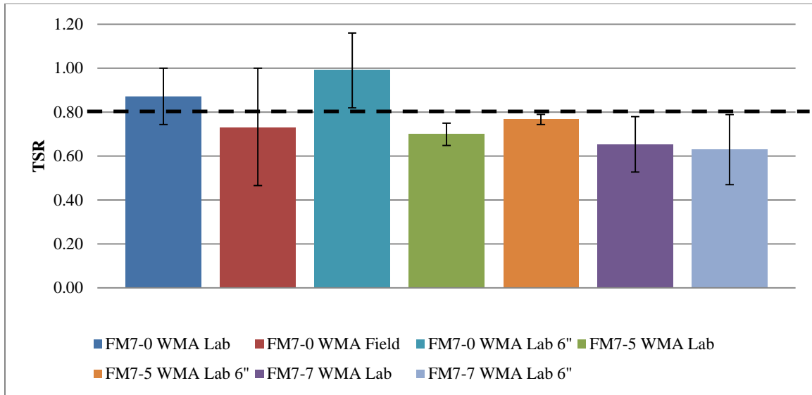
Figure 4.39 FM7 TSR results (Evotherm with 0%, 5%, and 7%)
