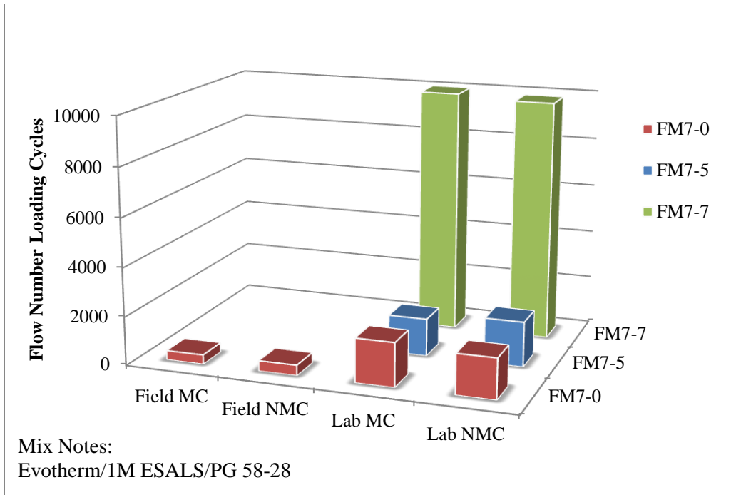
Figure 4.20 Flow number comparison for FM7
