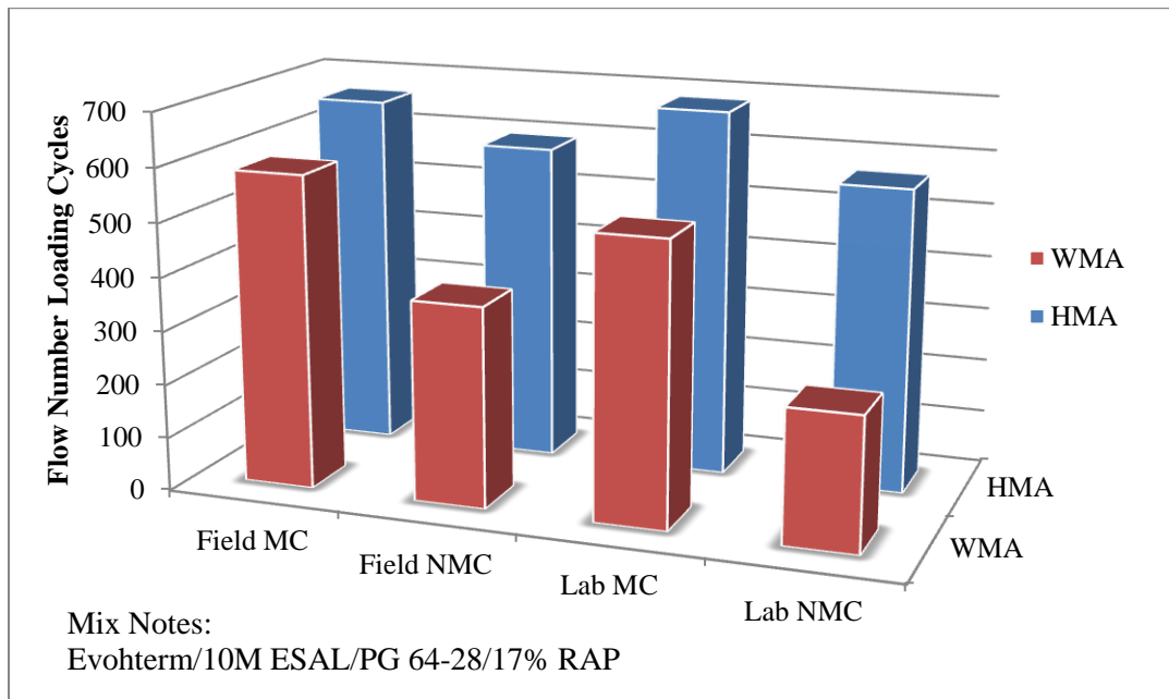
Figure 4.10 FM2 flow number comparison
