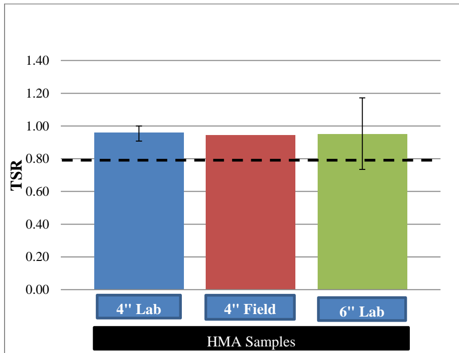
Figure 4.37 TSR values for FM6 (Evotherm)
