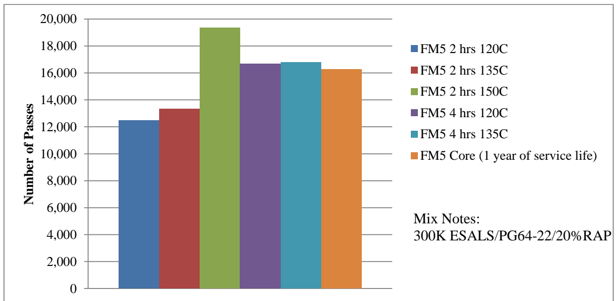
Figure 4.48 Stripping inflection point for FM5 comparing curing time and temperature (Average core air voids are 11.3%)
