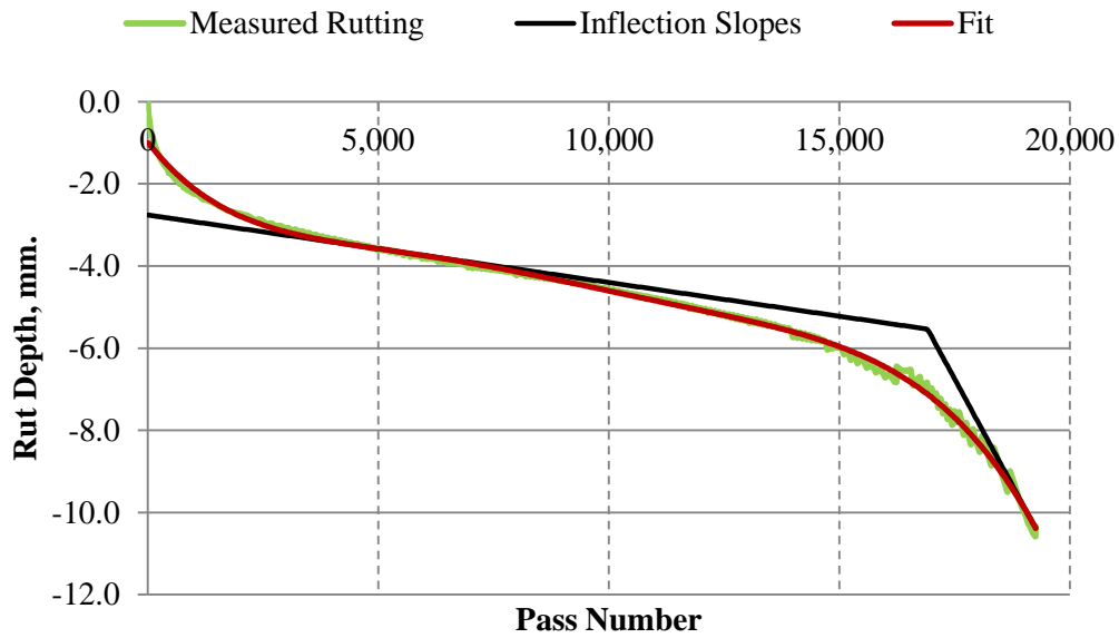
Figure 3.10 Hamburg wheel tracking test results
