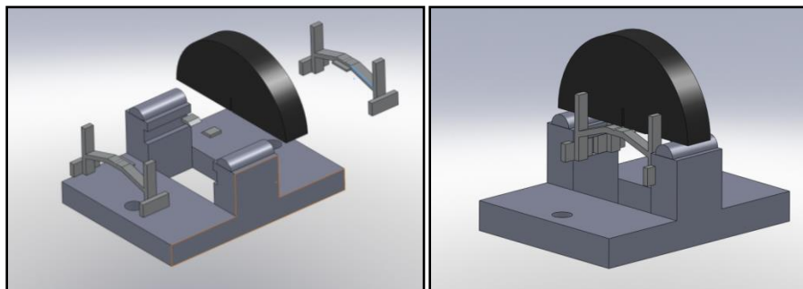
Figure 3.6 Loading frame designed at Iowa State University (Courtesy of Sheng Tang)
