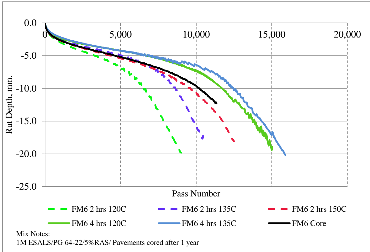
Figure 4.49 FM6 Hamburg wheel tracking test results with variable time and temperatures (Average core air voids are 7.1%)
