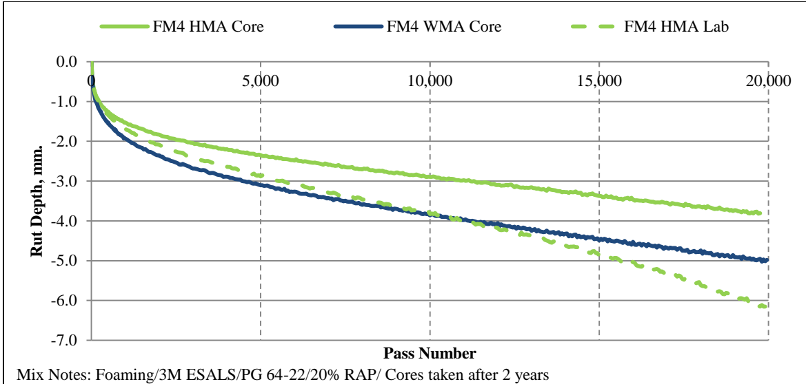
Figure 4.42 FM4 Hamburg rutting depth versus passes (HMA/Foam) (Average core air voids are HMA=5.8% and WMA=4.6%)
