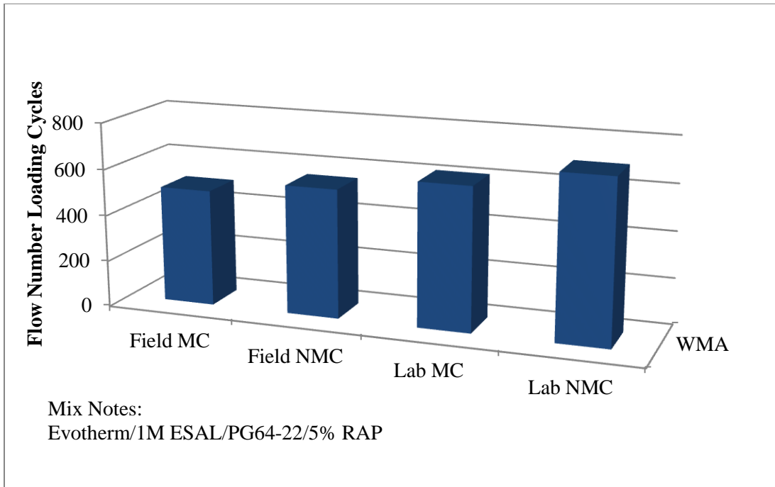
Figure 4.18 Flow number comparison for FM6
