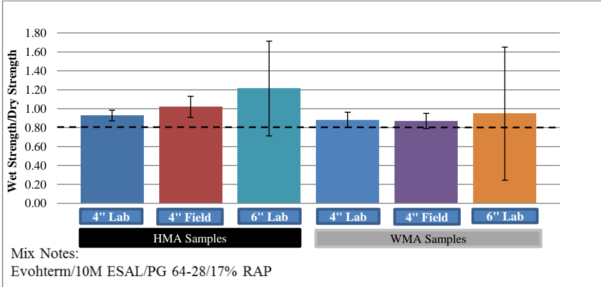
Figure 4.29 FM2 TSR results (HMA/Evotherm)
