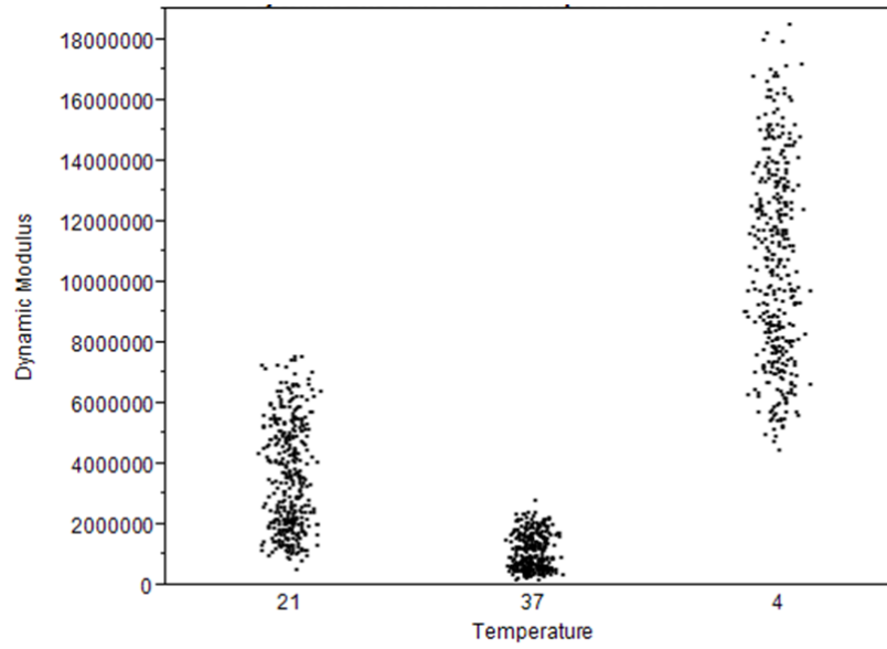
Figure 4.2 Non-transformed dynamic modulus data
