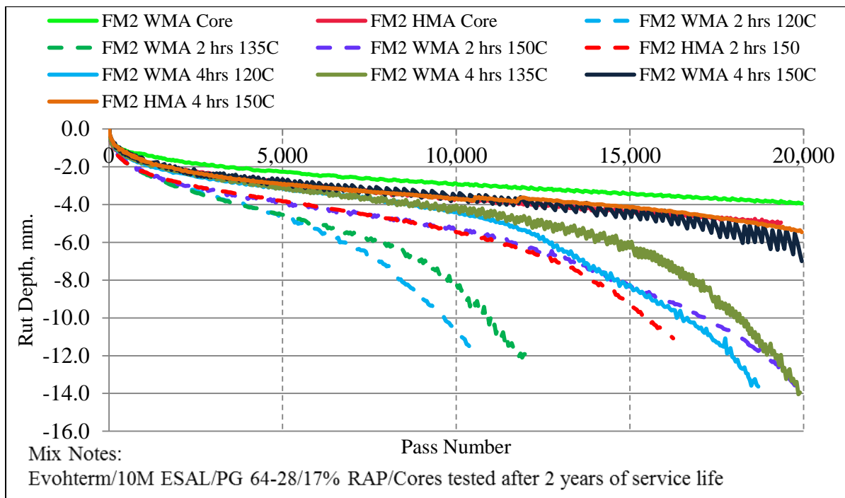
Figure 4.45 Hamburg results comparing curing temperature and time for FM2 HMA and WMA
