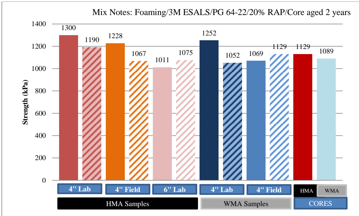
Figure 4.32 FM4 IDT peak strength (HMA/Foam) (Average core air voids are HMA=6.5% and WMA=5.2%)
