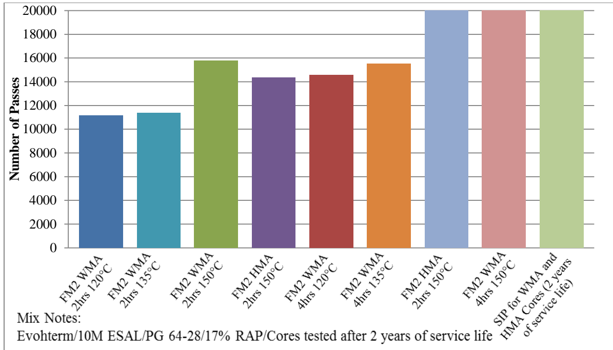
Figure 4.46 Stripping inflection point for FM2 comparing HMA with WMA, curing time and temperature (SIP for FM2 cores is 20,000) (Average core air voids are HMA=6.7% and WMA=7.1%)
