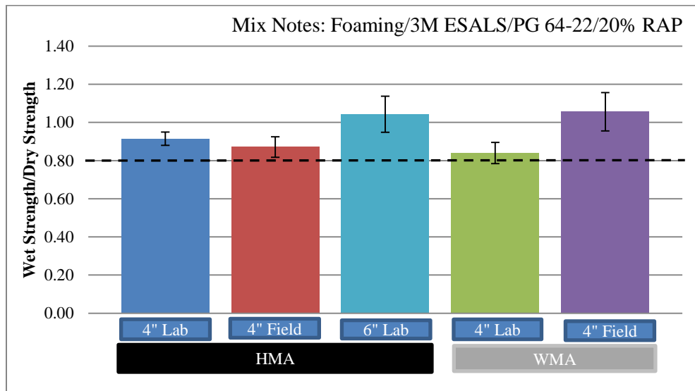
Figure 4.33 FM4 TSR results (HMA/Foam)
