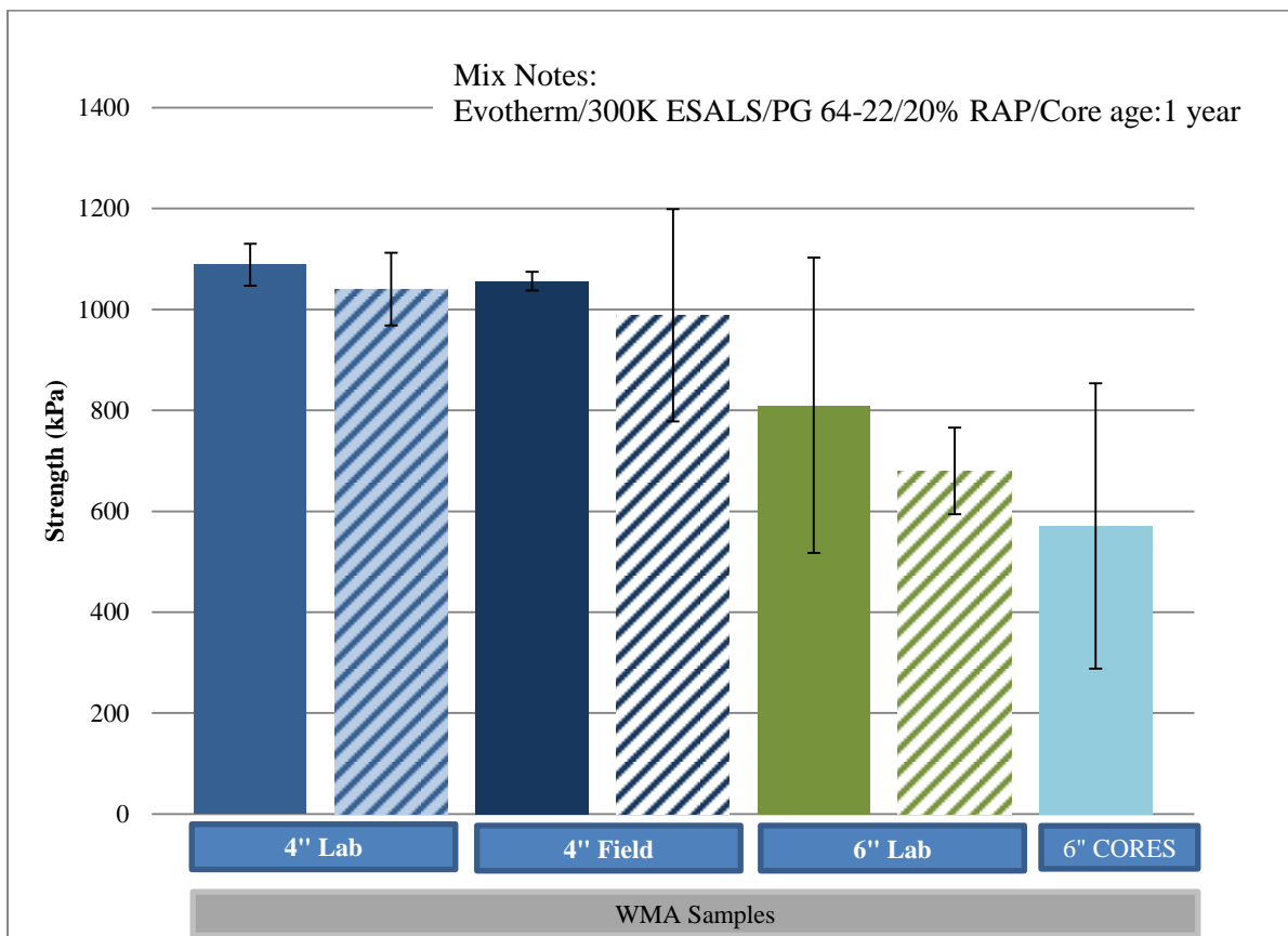
Figure 4.34 FM5 IDT peak strength (Evotherm) (Average core air voids are 9.3%)
