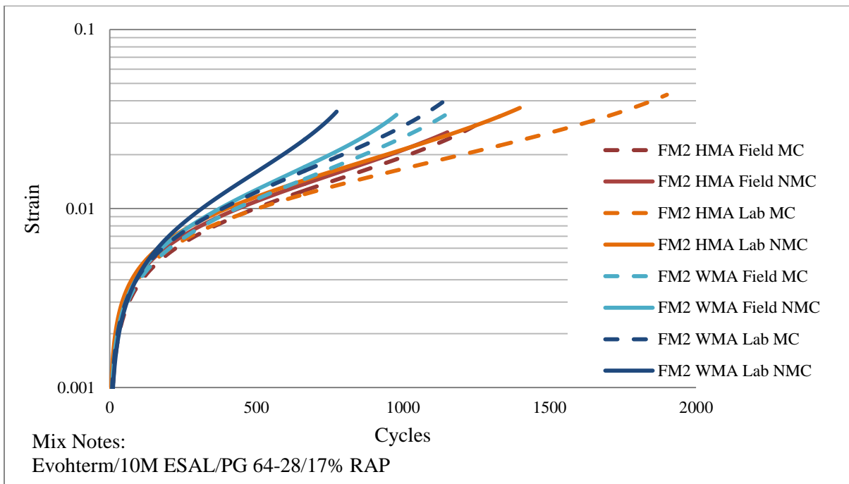
Figure 4.11 Strain versus cycles plot for FM2 (HMA/Evohterm)
