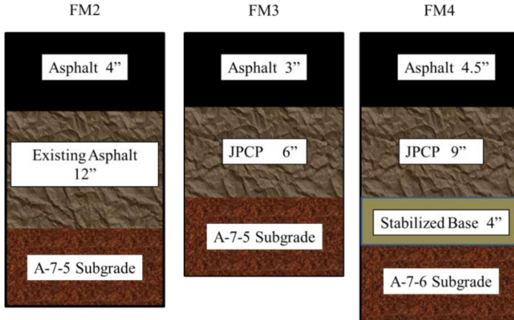
Figure 6.8 Pavement structures used in MEPDG analysis
