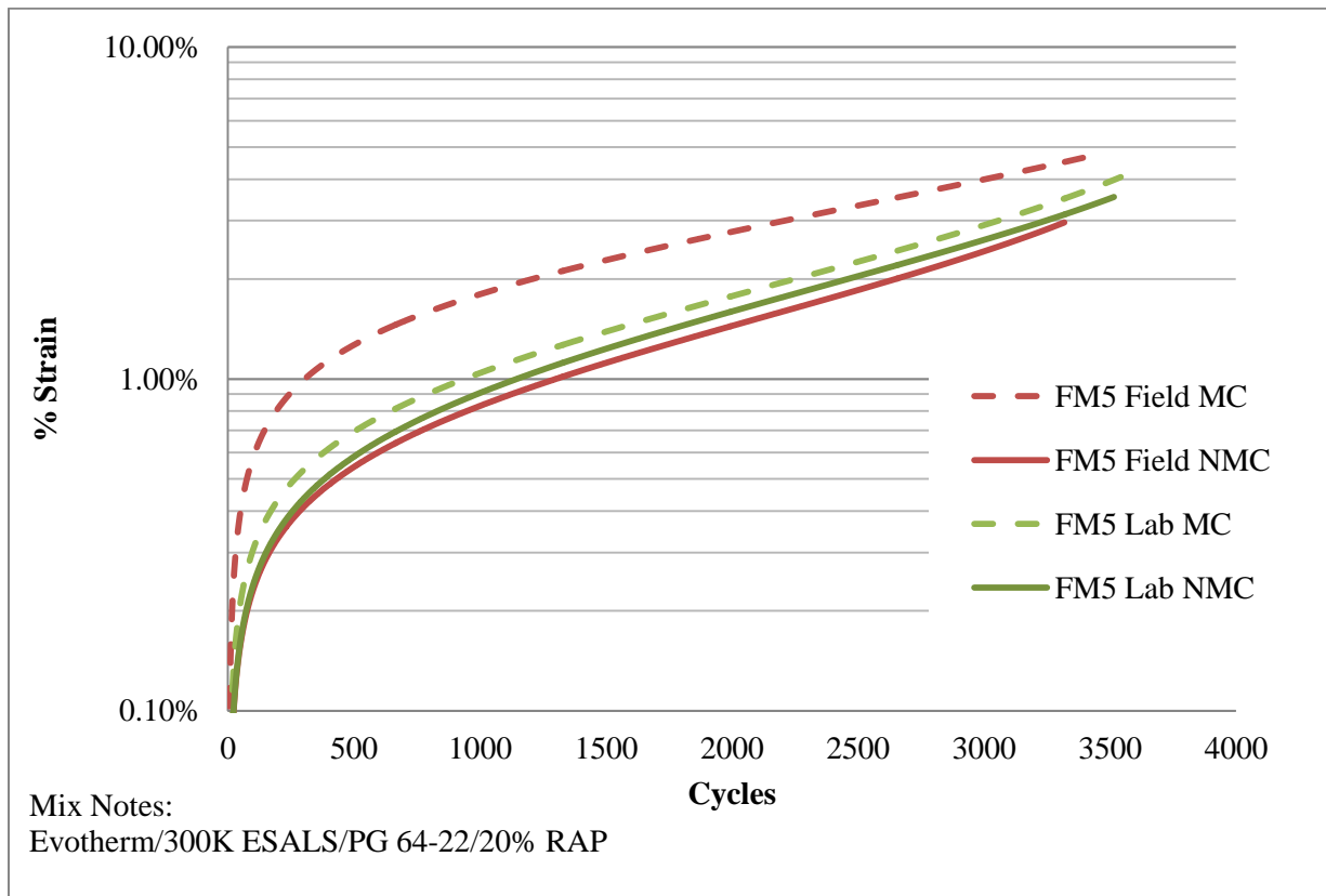
Figure 4.17 Strain versus cycles plot for FM5 (Evotherm)
