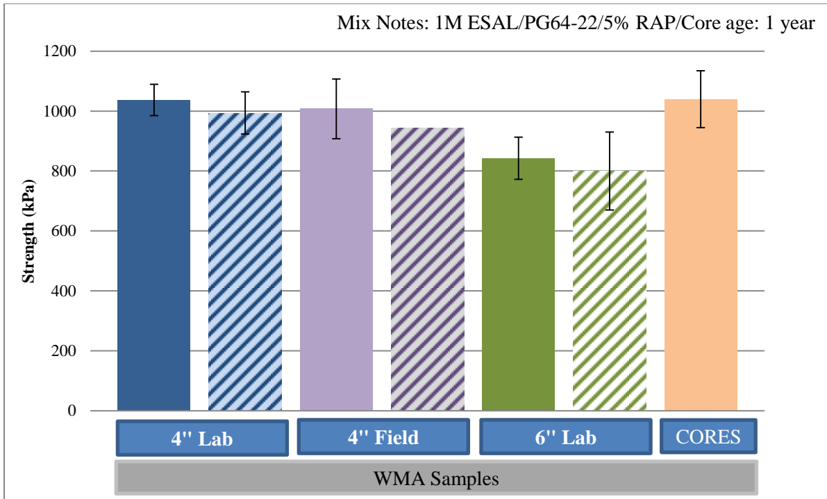
Figure 4.36 FM6 IDT peak strength (Evotherm) (Average core air voids are 8.0%)
