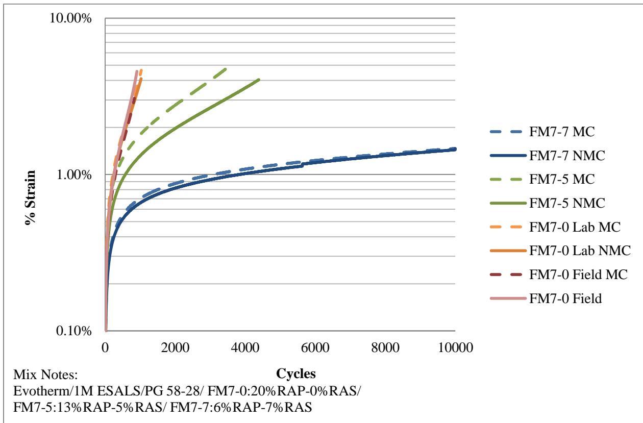
Figure 4.21 Strain versus cycles plot for FM7 (Evotherm and Shingles)
