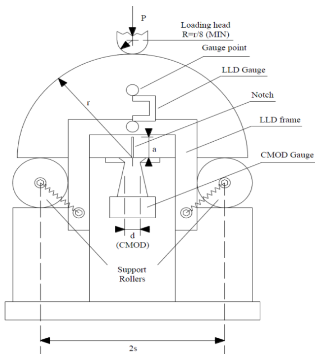
Figure 3.5 Original proposed loading frame for SCB testing (draft standard)
