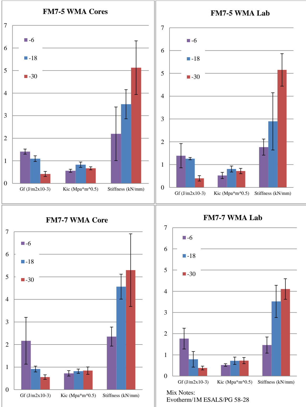
Figure 4.27 SCB results for FM7-5 and FM7-7 (Evotherm with 5% and 7% Shingles)
