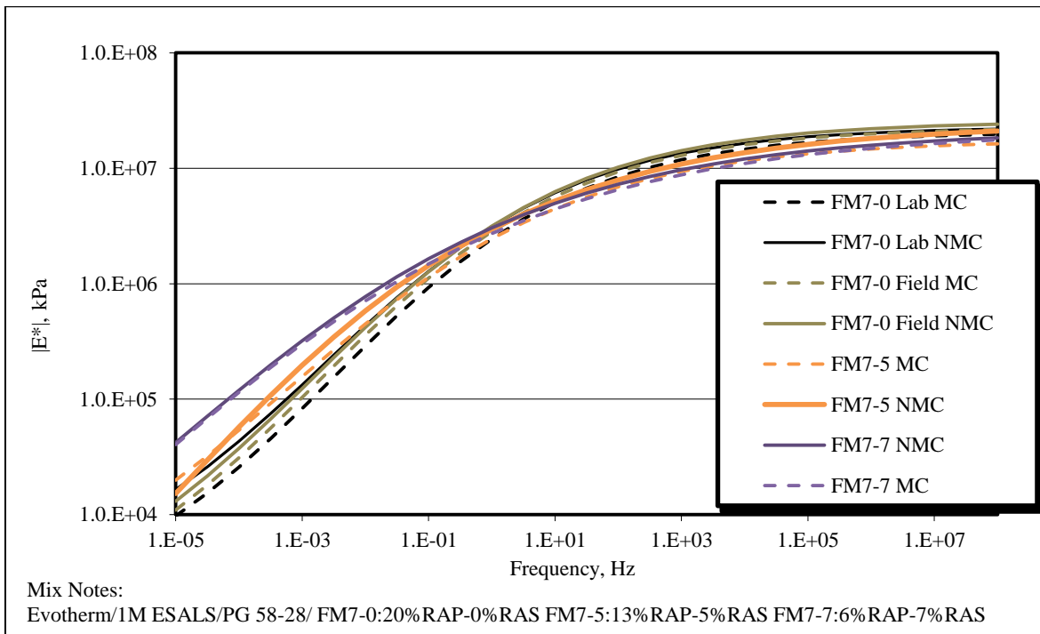
Figure 4.9 FM7 (Evotherm with 0%, 5%, 7% Shingles) dynamic modulus master curves
