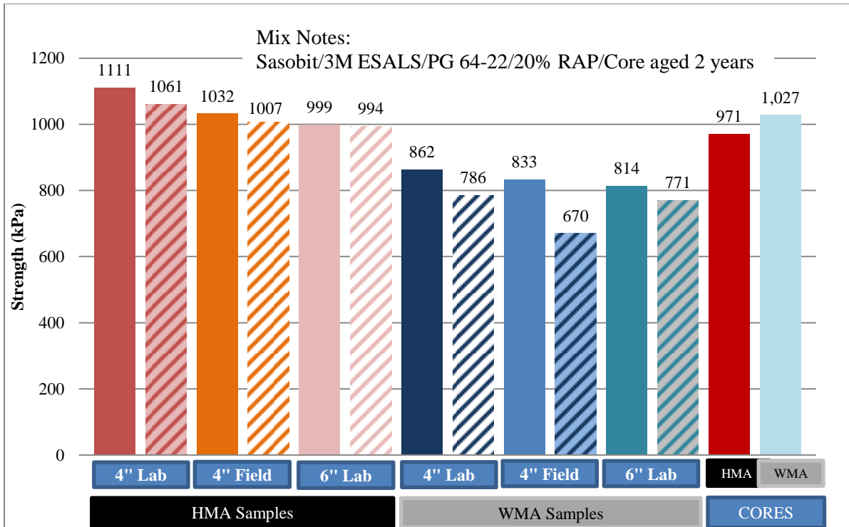
Figure 4.30 FM3 IDT peak strength (HMA/Sasobit) (Average core air voids are HMA=8.0% and WMA=7.8%)
